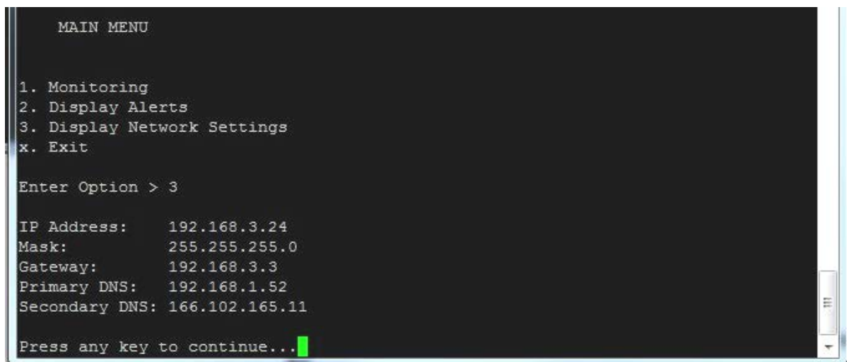
Figure 53- Text Menu-Network Settings
