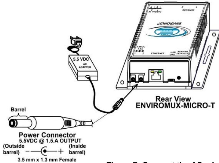
Figure 7- Connect the AC adapter and power-up
