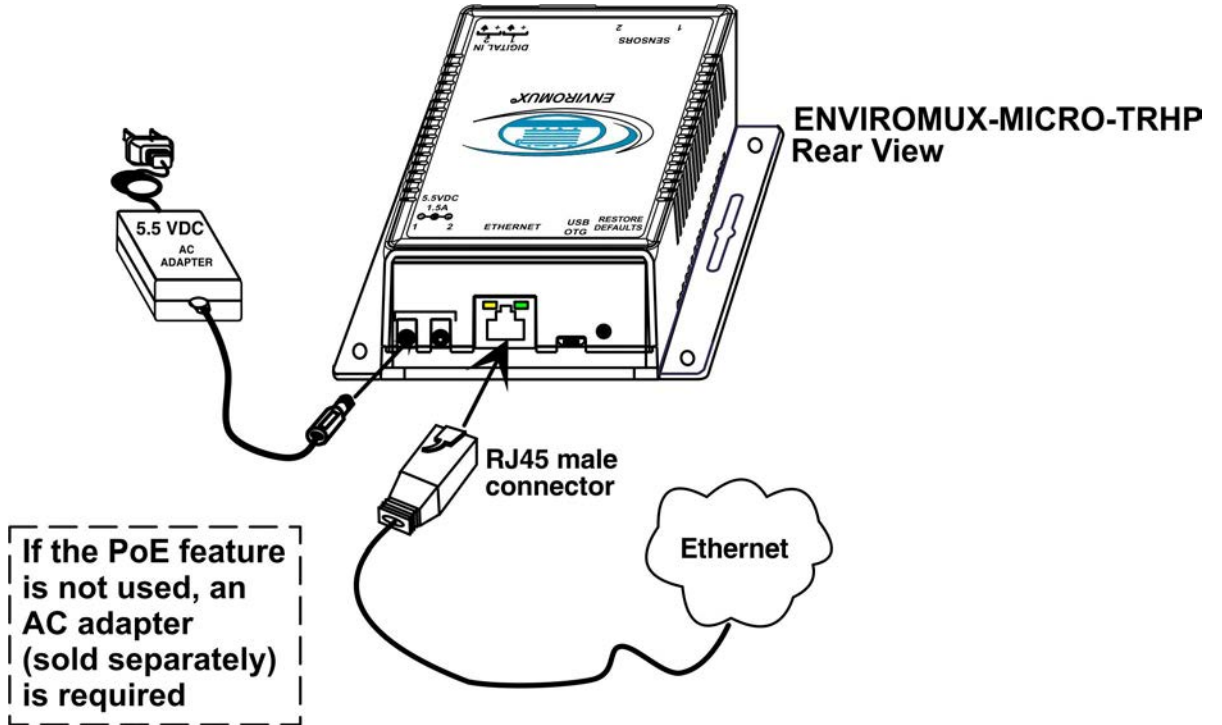
Figure 6- Connect ENVIROMUX-MICRO to the Ethernet
