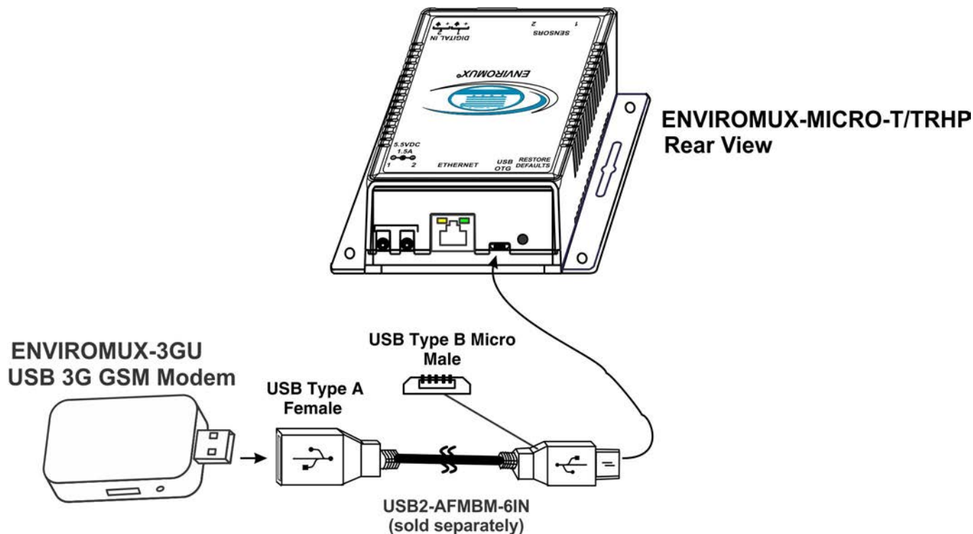
Figure 9- Connect a Modem
