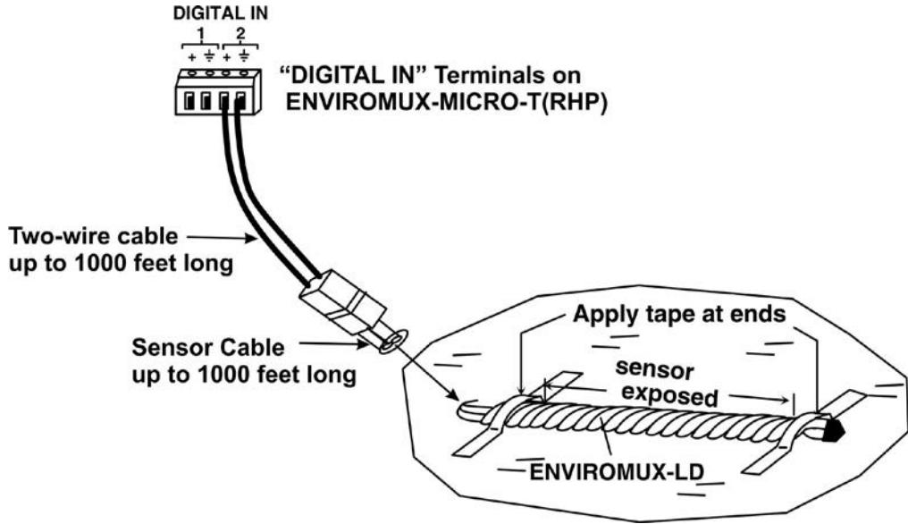
Figure 4- Secure liquid detection sensor with tape
